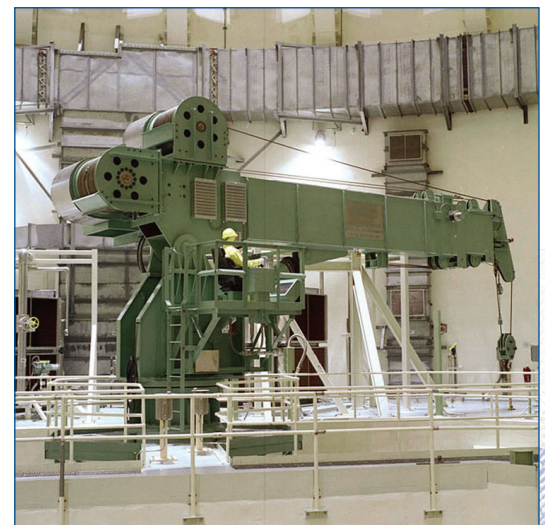
TELESCOPING JIB CRANE
