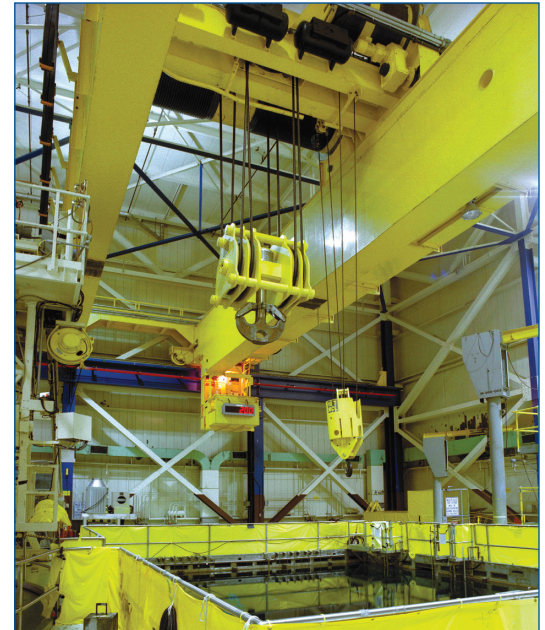
125 TON NUCLEAR FUEL HANDLING CRANE
